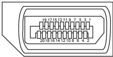
Figure 5. 20-pin DisplayPort
